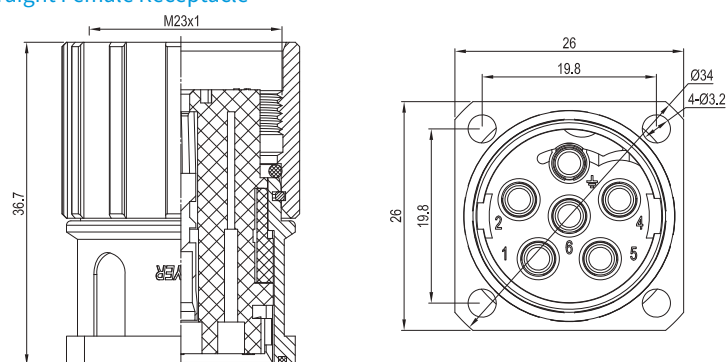
方座直式母插座 Square Straight Female Receptacle
