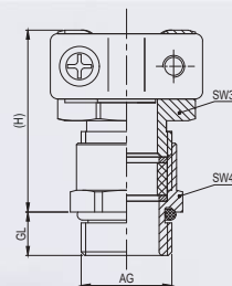
MPKM双锁紧型金属电缆防水接头 MPKM double-lock metal cable gland
