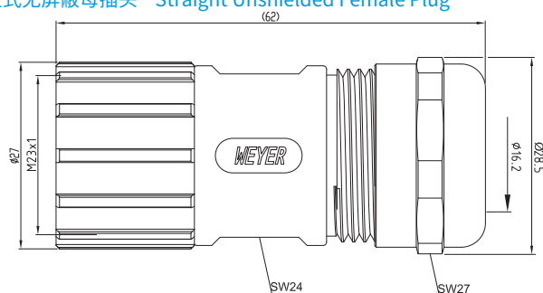
直式无屏蔽母插头 Straight Unshielded Female Plug
