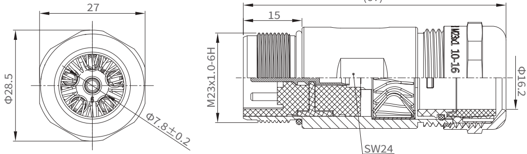
直式弹簧屏蔽公插座 Straight Shielded Male Receptacle
