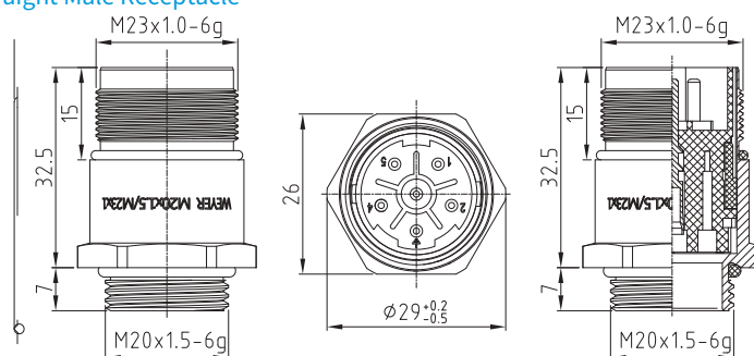
M20螺纹座直式公插座 M20 Straight Male Receptacle
