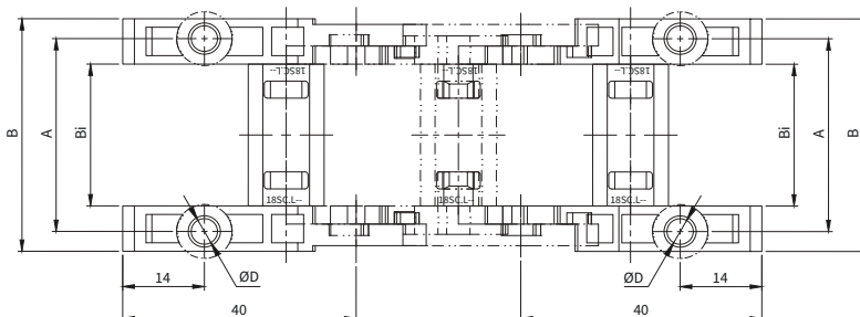
拖链安装接头 Installation of end connectors
