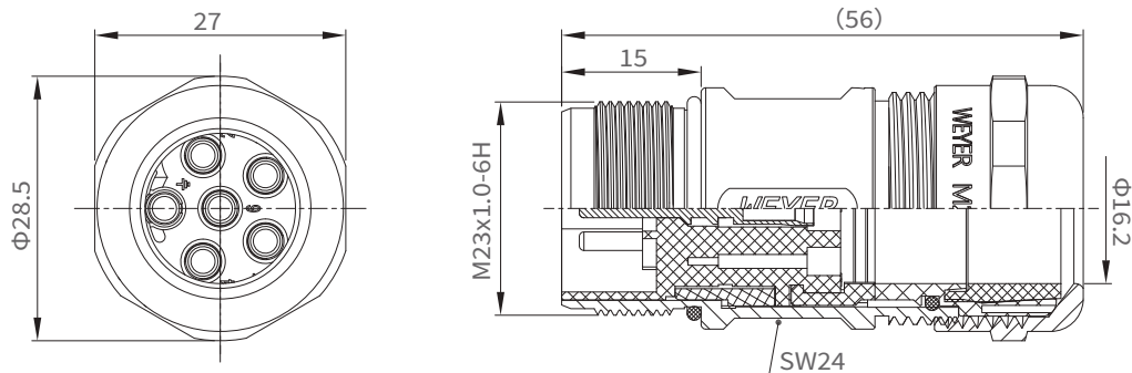
直式无屏蔽公插座 Straight Unshielded Male Receptacle
