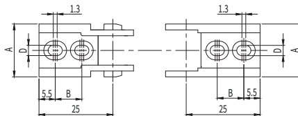
拖链安装接头 Installation of end connectors
