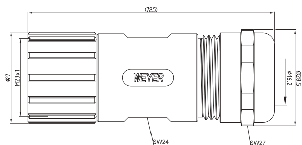
直式弹簧屏蔽母插头 Straight Shielded Female Plug
